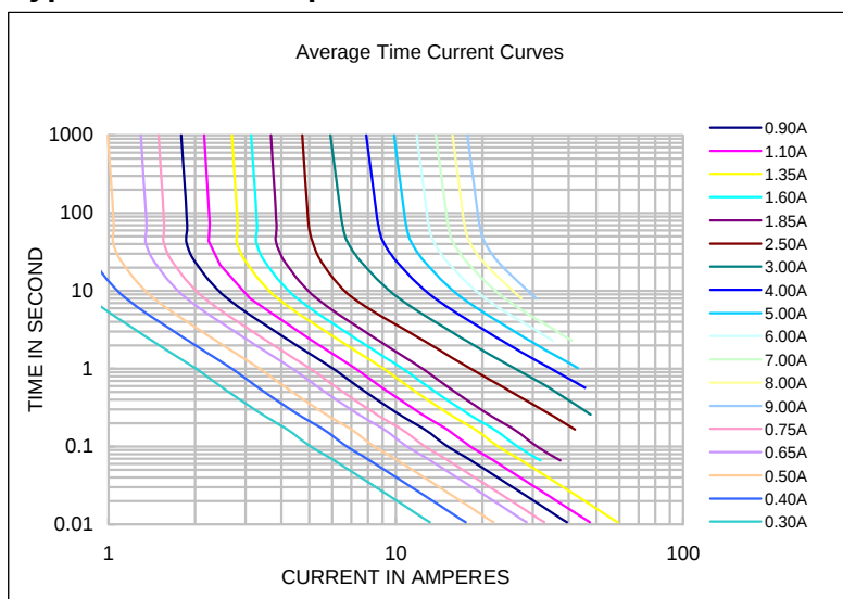
Typical Time-To-Trip Curve At 25°C
