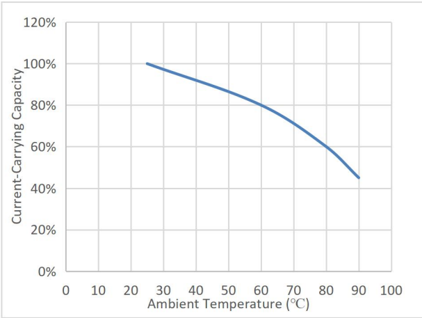
Current Carrying Capacity at various ambient temperature
