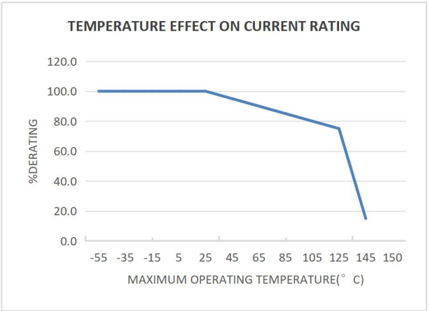
Current Carrying Capacity at various ambient temperature
