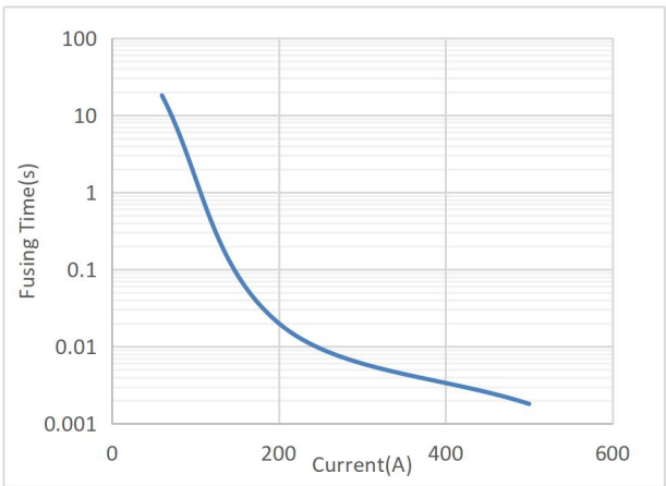
Various interrupting current at 25℃ ambient temperature
