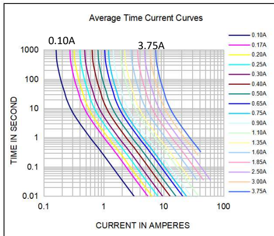
Typical time-to-trip curve at 25°C
